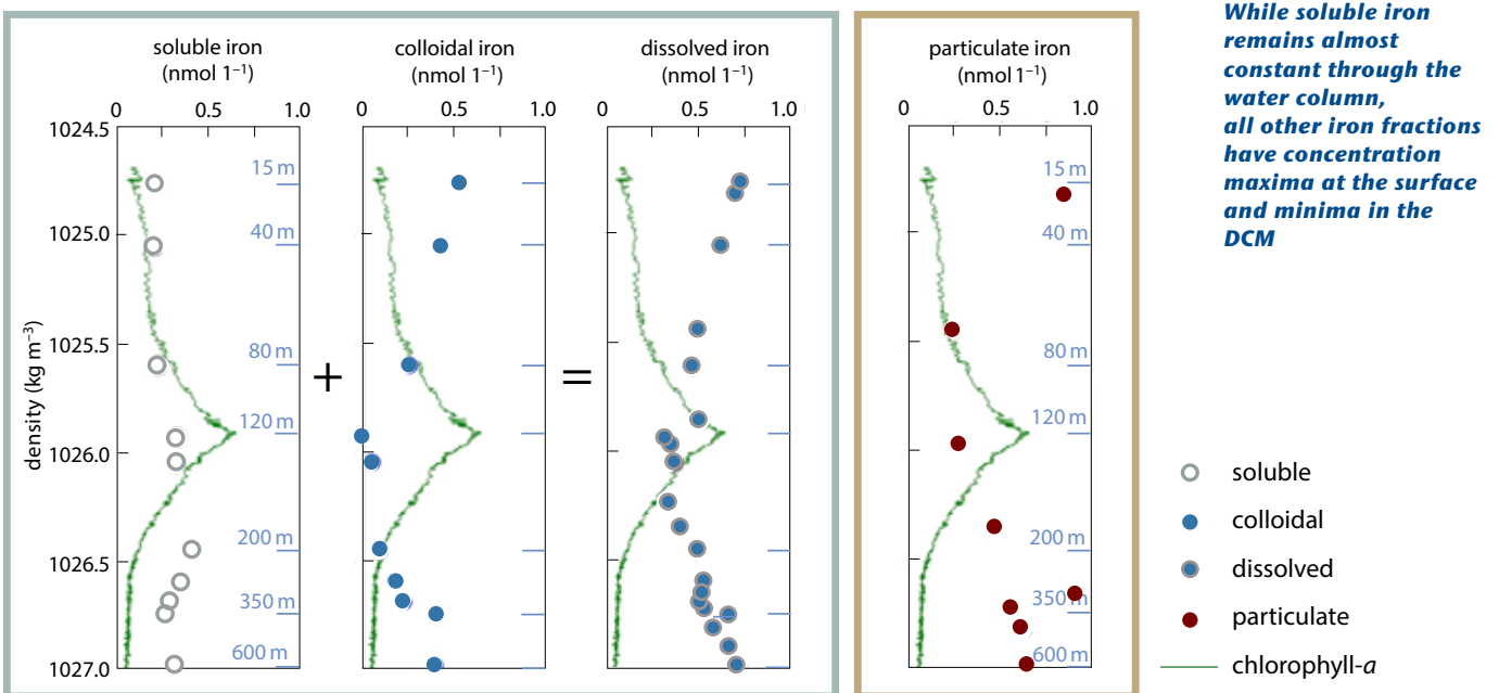
Figure 5 Representative upper ocean profiles (down to approximately 600 m) of soluble, colloidal, dissolved and particulate iron concentrations against density from the central North Atlantic (23°N, 40°W) during summer 2017. Approximate corresponding depths are shown in blue on the right-hand axes. The green line shows the chlorophyll-a concentration (in arbitrary units), a rough measure of biomass, and its peak is the deep chlorophyll-a maximum (DCM). (Data from Kunde et al., 2019)
