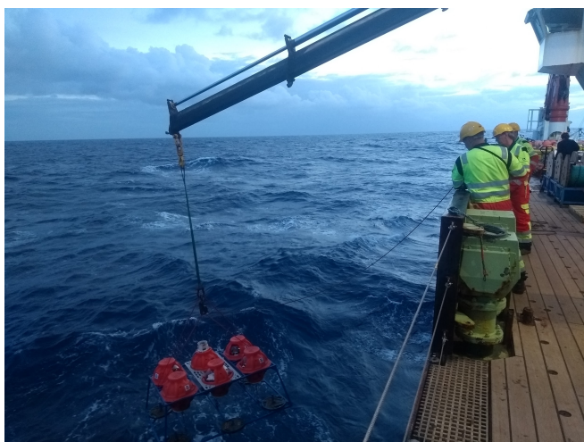
Deploying one of two PIES arrays. Credit: Matt Clark
